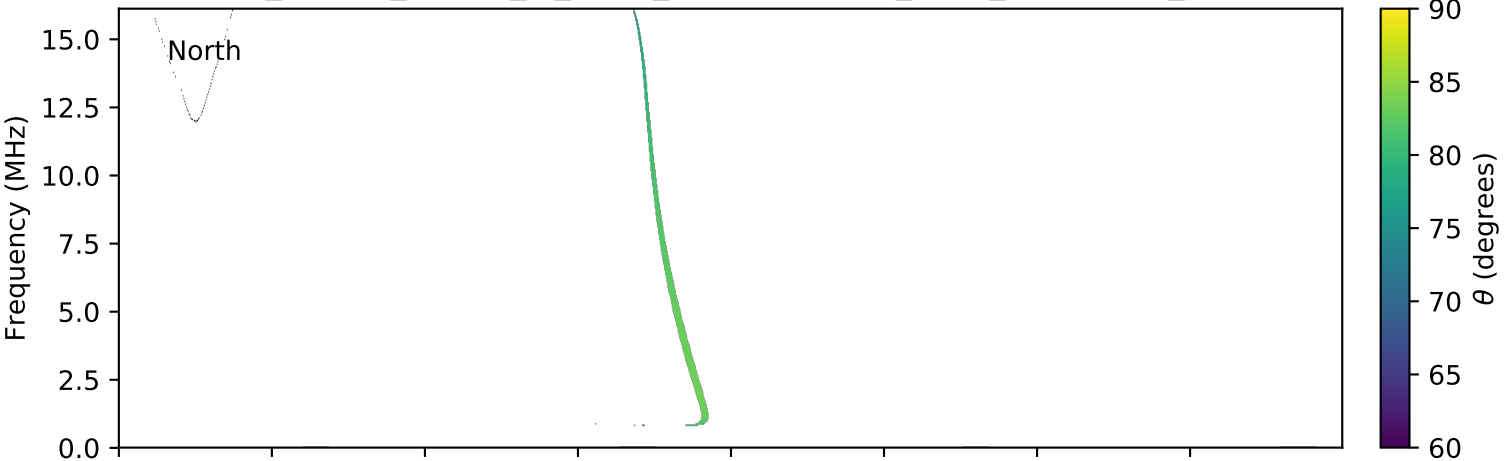
expres_cassini_jupiter_io_isaac_lossc-wid1deg_3kev_20000113_v01.cdf
