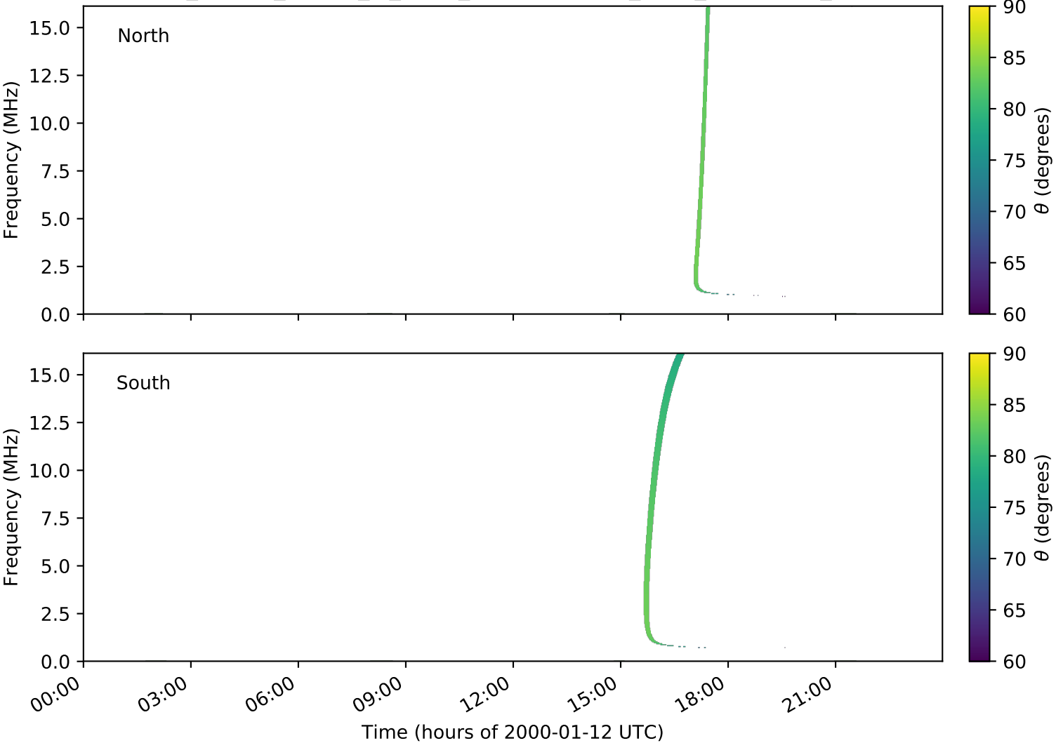
expres_cassini_jupiter_io_isaac_lossc-wid1deg_3kev_20000112_v01.cdf
