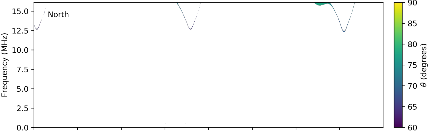
expres_cassini_jupiter_ganymede_isaac_lossc-wid1deg_3kev_20000130_v01.cdf
