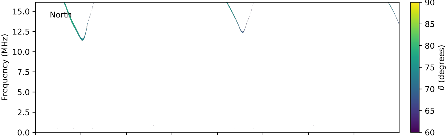
expres_cassini_jupiter_ganymede_isaac_lossc-wid1deg_3kev_20000129_v01.cdf
