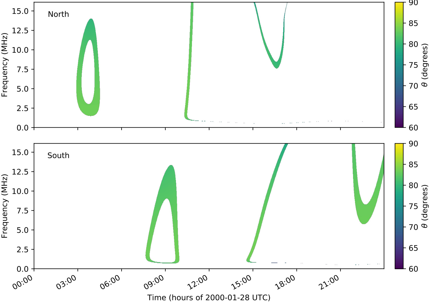
expres_cassini_jupiter_ganymede_isaac_lossc-wid1deg_3kev_20000128_v01.cdf
