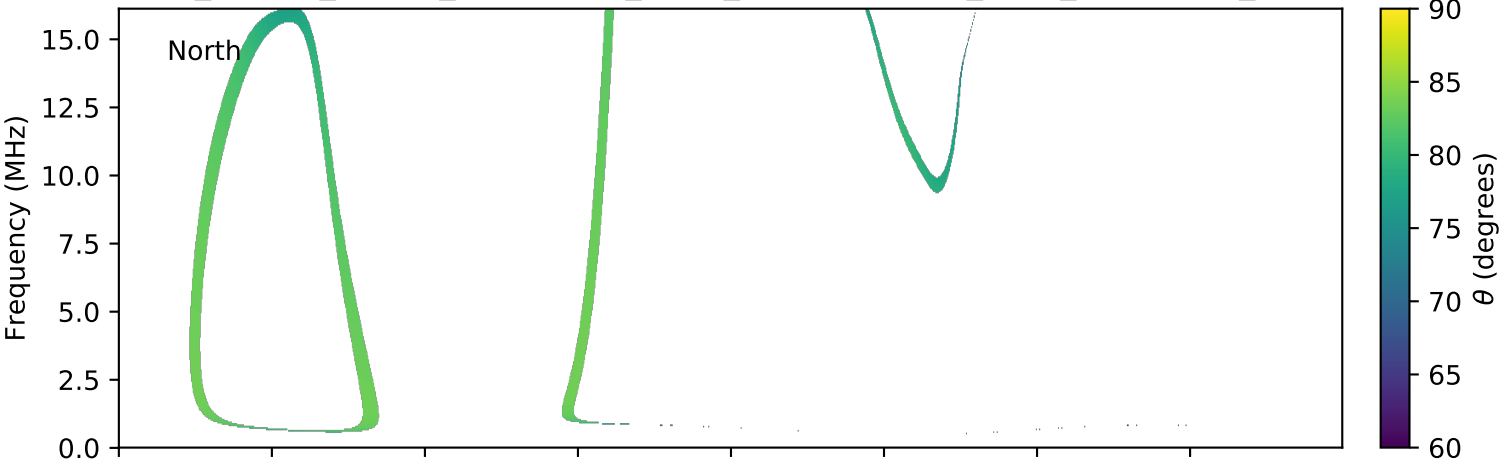
expres_cassini_jupiter_ganymede_isaac_lossc-wid1deg_3kev_20000121_v01.cdf
