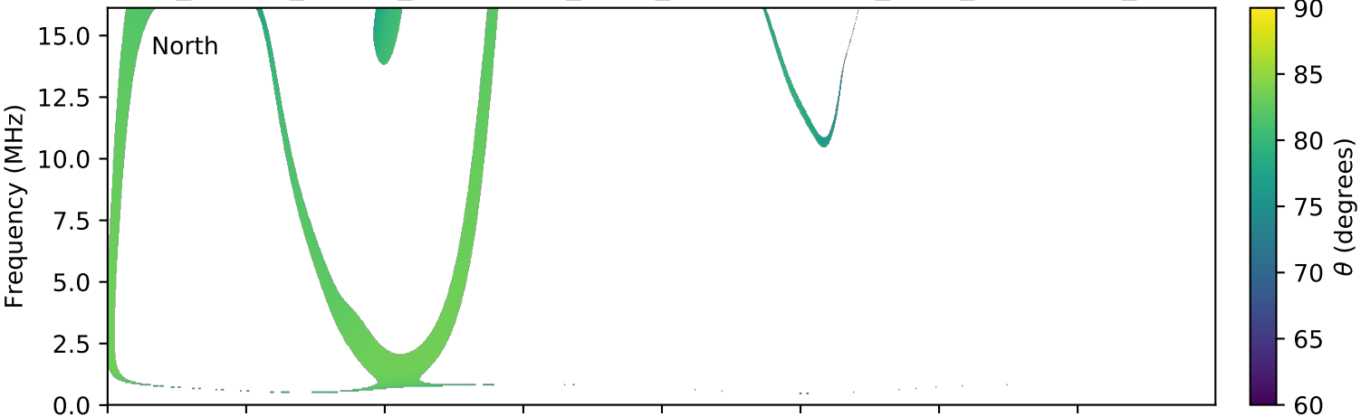
expres_cassini_jupiter_ganymede_isaac_lossc-wid1deg_3kev_20000114_v01.cdf
