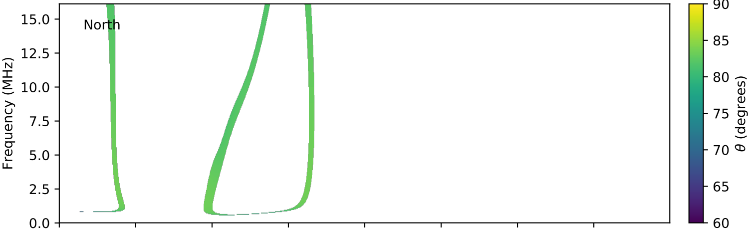
expres_cassini_jupiter_ganymede_isaac_lossc-wid1deg_3kev_20000110_v01.cdf
