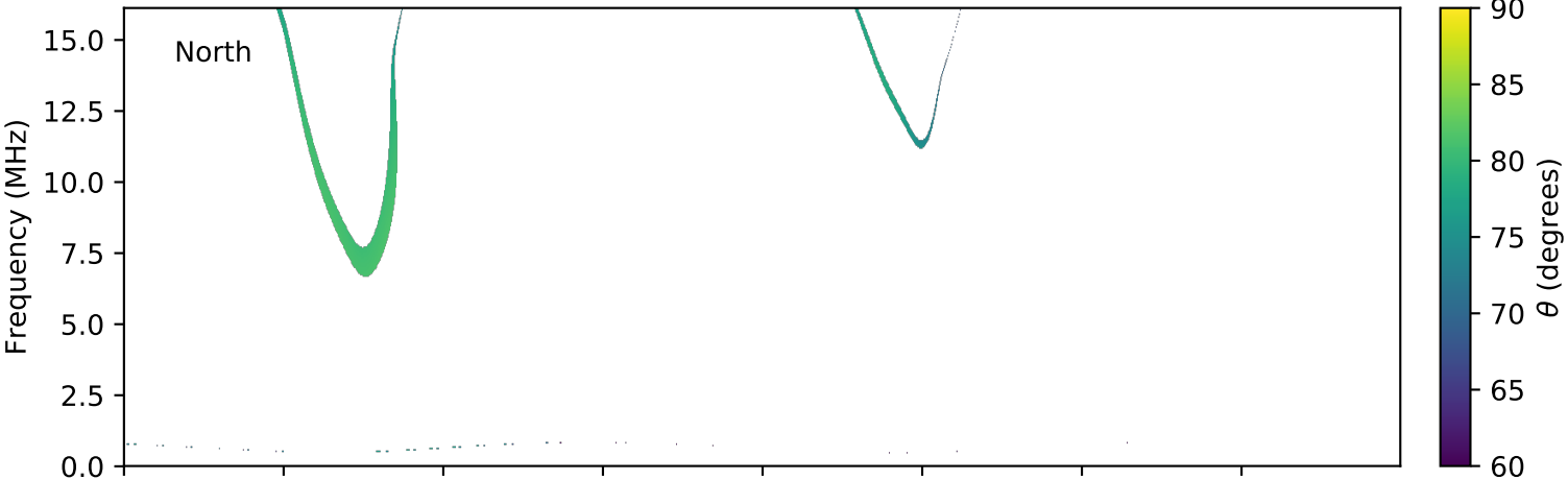
expres_cassini_jupiter_ganymede_isaac_lossc-wid1deg_3kev_20000107_v01.cdf
