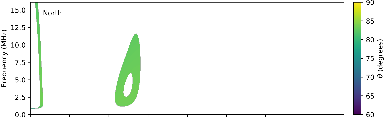
expres_cassini_jupiter_ganymede_isaac_lossc-wid1deg_3kev_20000103_v01.cdf
