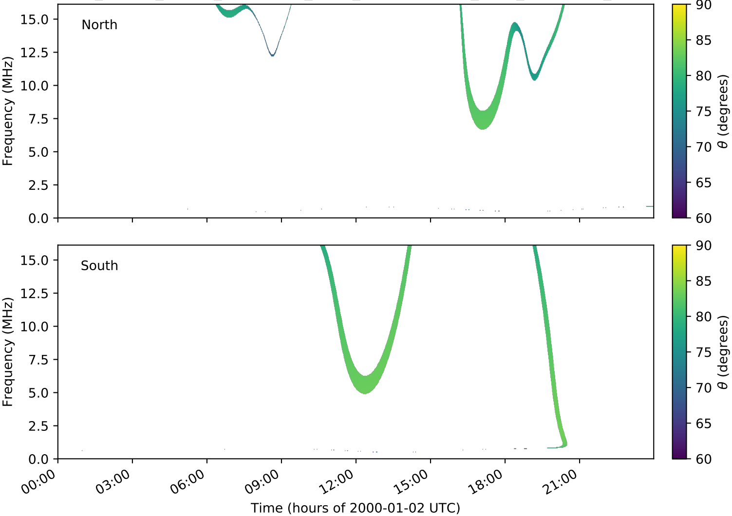
expres_cassini_jupiter_ganymede_isaac_lossc-wid1deg_3kev_20000102_v01.cdf
