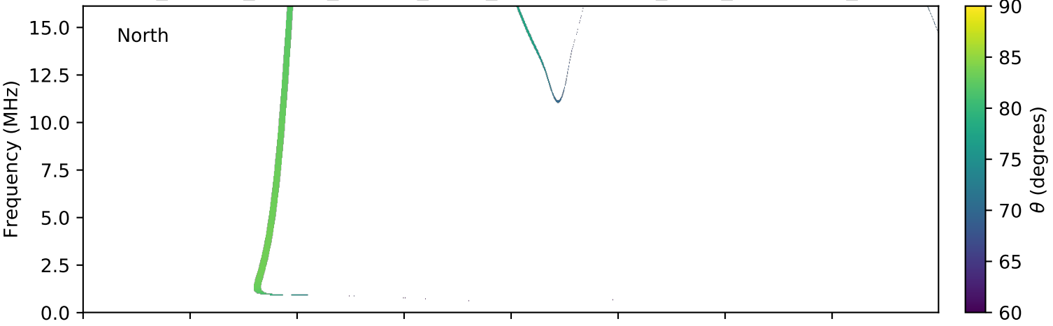
expres_cassini_jupiter_europa_isaac_lossc-wid1deg_3kev_20000129_v01.cdf
