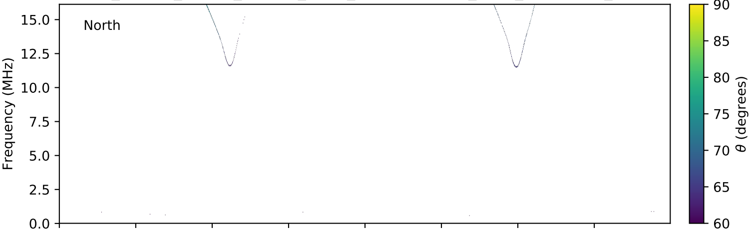
expres_cassini_jupiter_europa_isaac_lossc-wid1deg_3kev_20000126_v01.cdf
