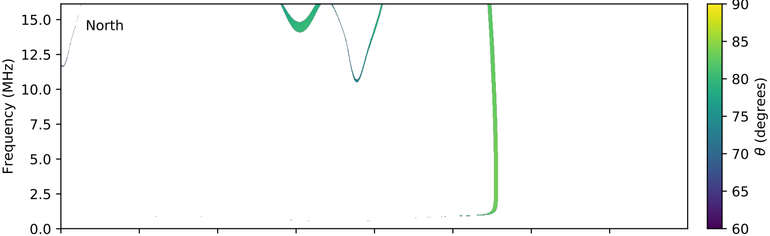
expres_cassini_jupiter_europa_isaac_lossc-wid1deg_3kev_20000123_v01.cdf
