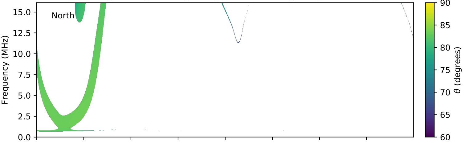
expres_cassini_jupiter_europa_isaac_lossc-wid1deg_3kev_20000122_v01.cdf
