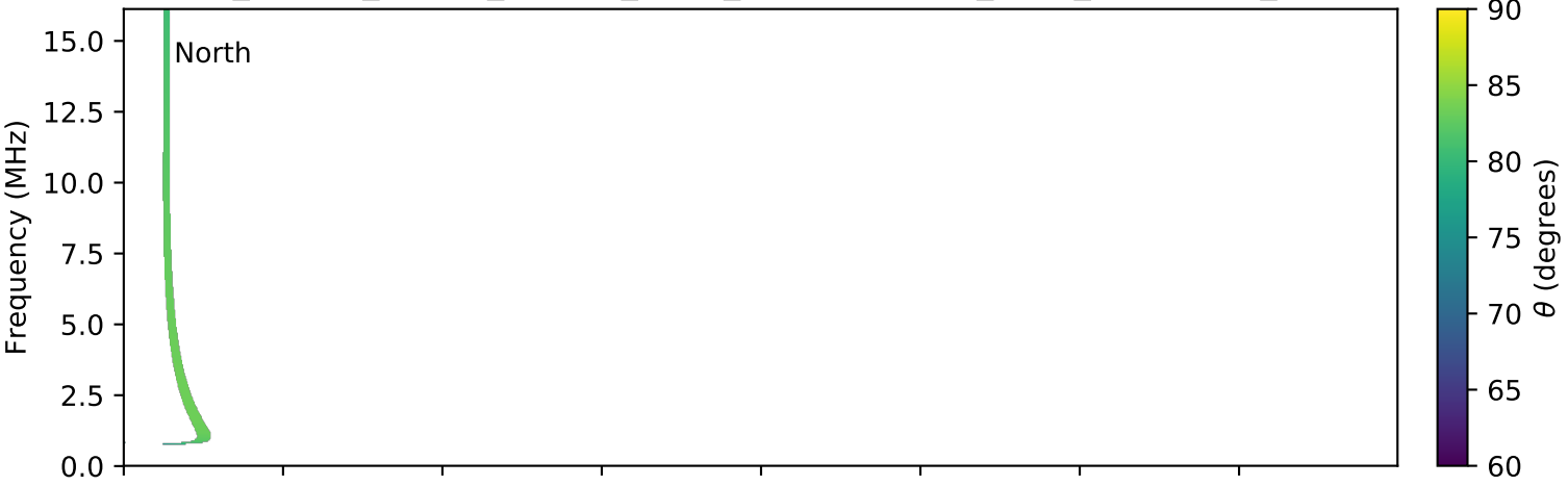
expres_cassini_jupiter_europa_isaac_lossc-wid1deg_3kev_20000120_v01.cdf
