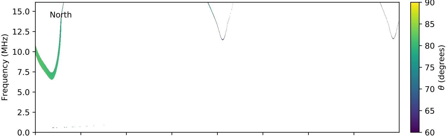
expres_cassini_jupiter_europa_isaac_lossc-wid1deg_3kev_20000115_v01.cdf
