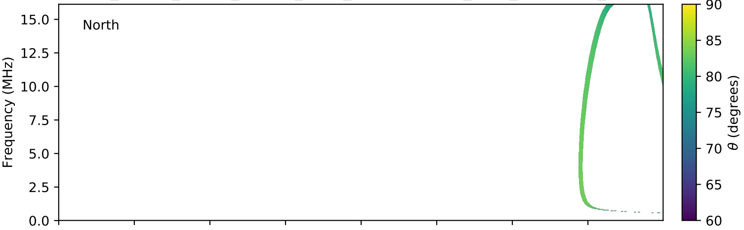
expres_cassini_jupiter_europa_isaac_lossc-wid1deg_3kev_20000114_v01.cdf
