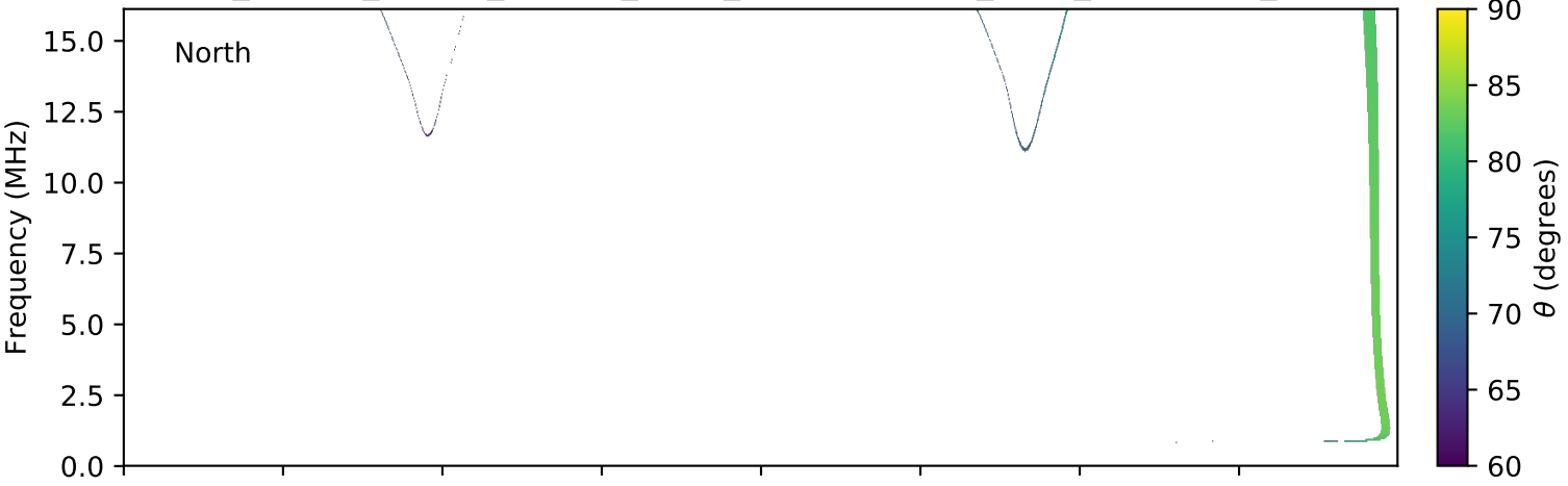
expres_cassini_jupiter_europa_isaac_lossc-wid1deg_3kev_20000112_v01.cdf
