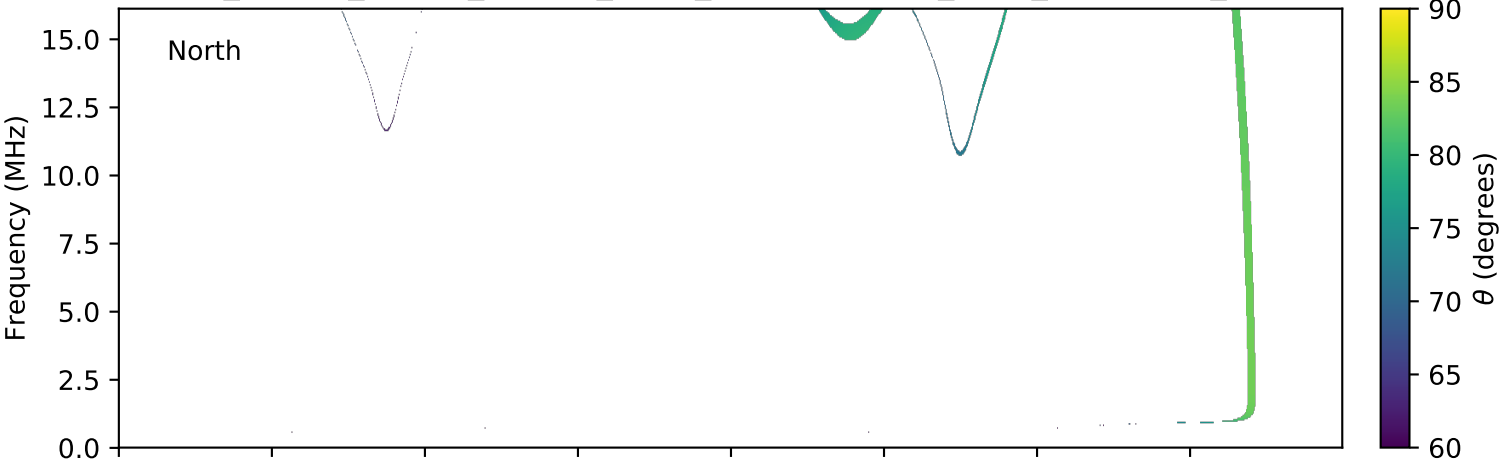
expres_cassini_jupiter_europa_isaac_lossc-wid1deg_3kev_20000105_v01.cdf
