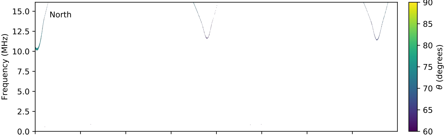
expres_cassini_jupiter_europa_isaac_lossc-wid1deg_3kev_20000101_v01.cdf
